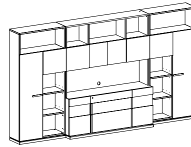
LIBRARY COMPOSITION 1 inch W 150" D 21" H 84" cm L 379,6 P 52,7 H 213,4 Crts 11 kg 414 m 3 2,048
