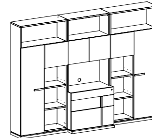
LIBRARY COMPOSITION 9 inch W 114" D 21" H 84" cm L 290 P 52,7 H 213,4 Crts 9 kg 316 m 3 1,396
