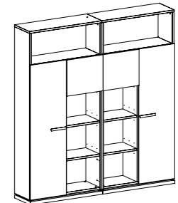
LIBRARY COMPOSITION 12 inch W 79" D 21" H 84" cm L 200 P 38,8 H 213,4 Crts 6 kg 200 m 3 0,786
