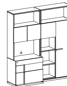
LIBRARY COMPOSITION 15 inch W 75" D 21" H 84" cm L 190 P 52,7 H 213,4 Crts 6 kg 216 m 3 1,003
