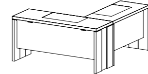
DESK COMPOSITION 2 Desk + Return desk inch W 66" D 71" H 30" cm L 167,5 P 175 H 76 Crts 2 kg 94 m 3 0,285
