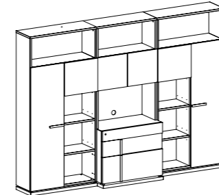
LIBRARY COMPOSITION 10 inch W 114" D 21" H 84" cm L 290 P 52,7 H 213,4 Crts 9 kg 316 m 3 1,396
